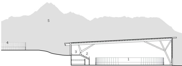
Cross section 1. New rink. 2. Seating area. 3. Concourse. 4. Demolished rink. 5. Roche de Boule mountain.
