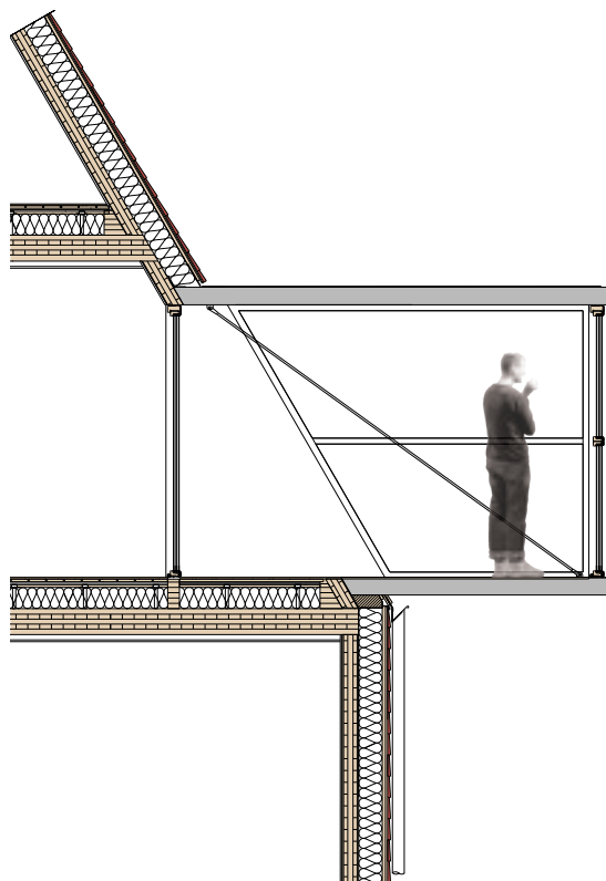
Structural detail.
