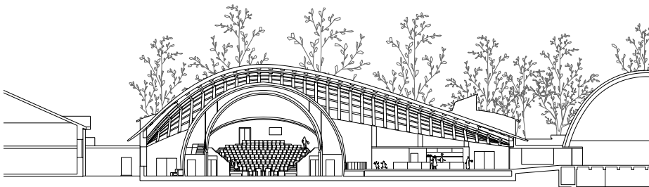
Cross-section
